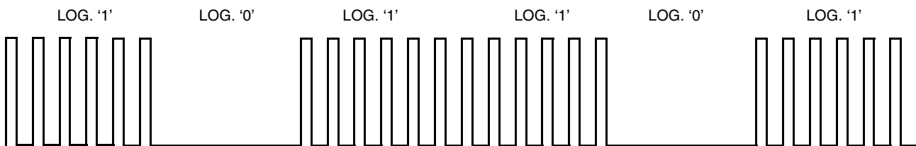
Figure 4. Pulse Position Encoding
